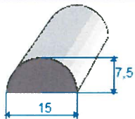
EPDM SPONGE RUBBER BLACK ROLLS OF 100 m REF 400120
