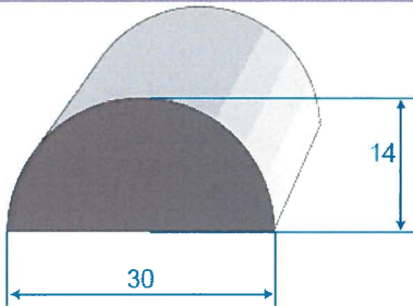
EPDM SPONGE RUBBER BLACK ROLLS OF 25 m REF 400082
