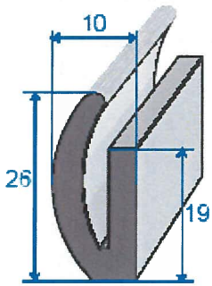
EPDM SPONGE RUBBER BLACK ROLLS OF 25 m REF 400082
