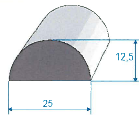
EPDM SPONGE RUBBER BLACK ROLLS OF 25 m REF 400116
