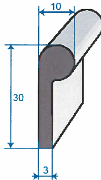
EPDM SPONGE RUBBER BLACK ROLLS OF 25 m REF 400046
